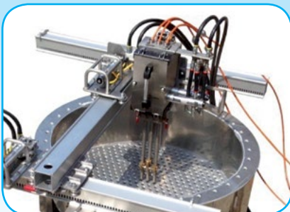
Automatic tube bundle blaster
